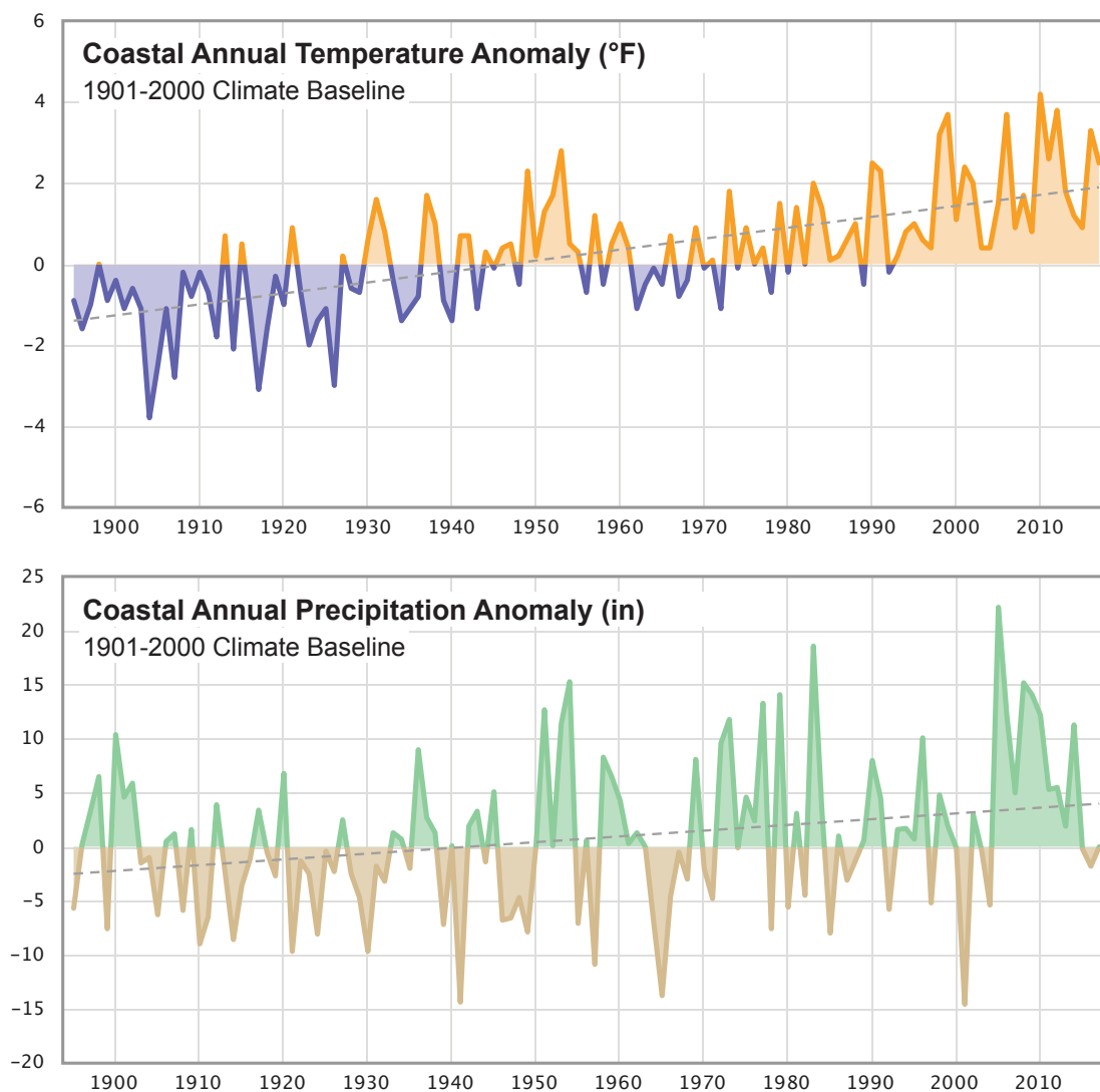
Figure 1. Maine coastal climate division annual temperature and precipitation 1895–2017. Dashed gray lines show long-term linear trends. Data from the NOAA U.S. Climate Divisional Dataset ( https://www.ncdc.noaa.gov/cag/ ).
